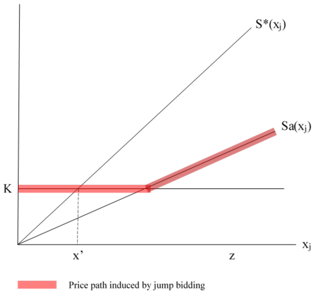
Figure 1: Symmetric equilibrium with jump bids
